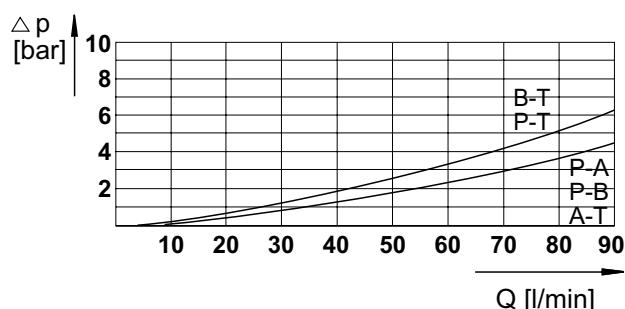
Characteristic curve for hydraulic oil 35 mm 2 /s, 50°C
